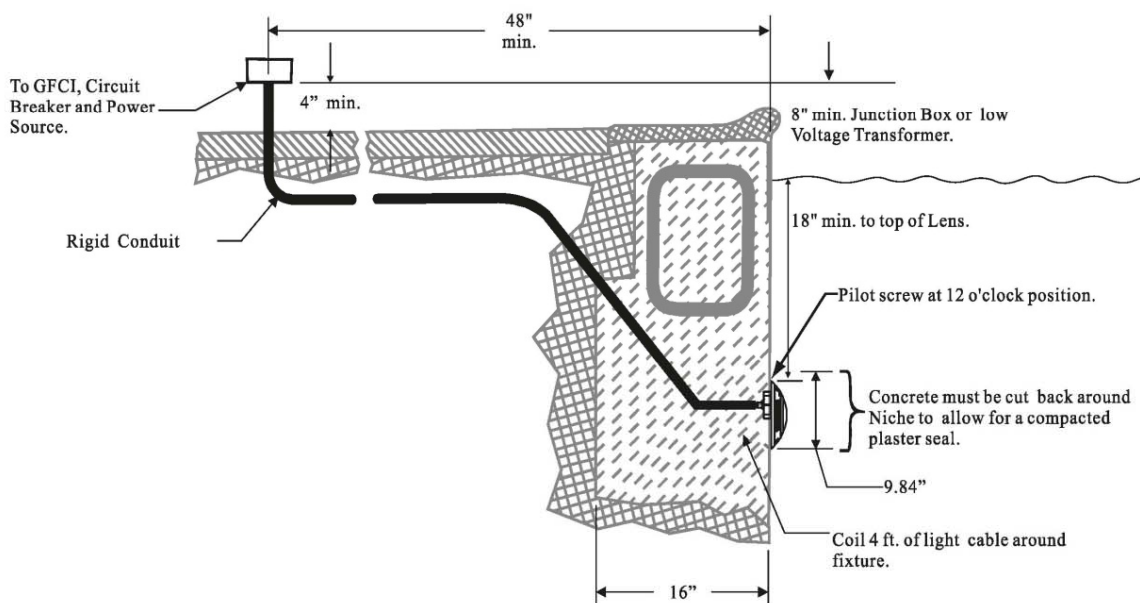
Installation Diagram for NS75 / NS150 Series
